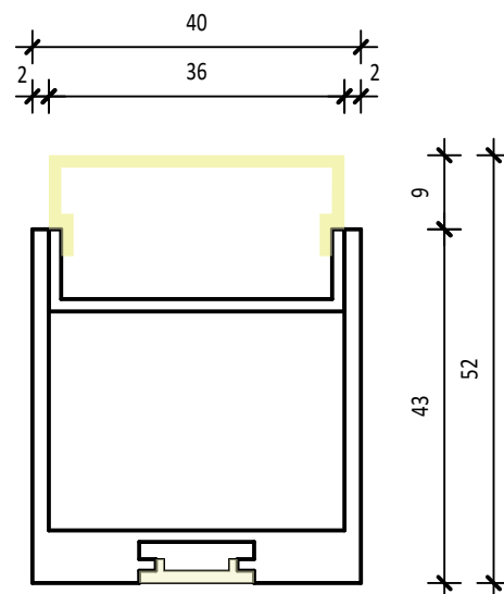
Diffusor 11.4mm
