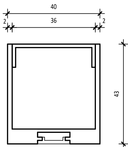
Diffusor BLIND
