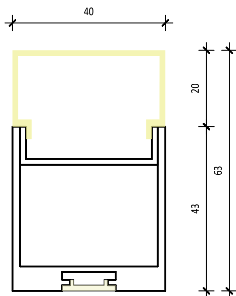
Diffusor 20mm
